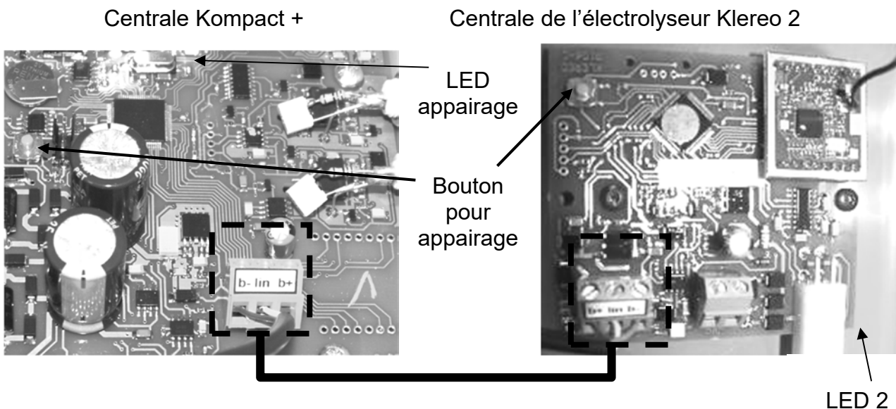
Figure 43. Branchement du bus de communication K-link
